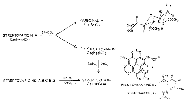
Figure 7. Degradation products derived from the streptovaricins.
