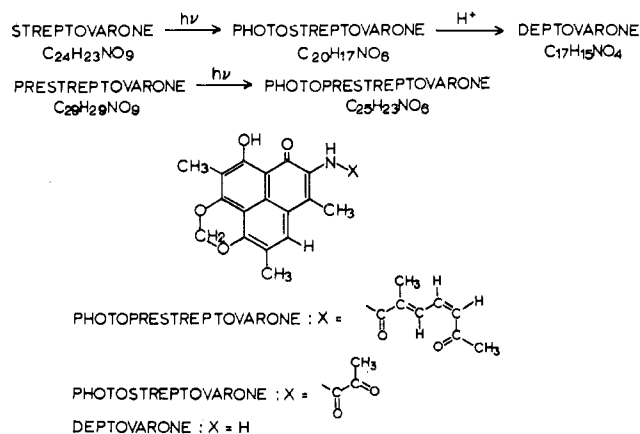
Figure 10. Structures of photostreptovarone and related products.
