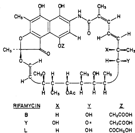
Figure 1. Structures assigned to rifamycins.
