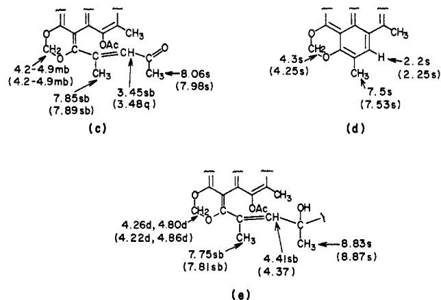
Figure 9. Chemical shifts of characteristic protons of streptovaricins and their degradation products: (a) 3-oxo- trans -2-pentenoic acid, (b) dapmavarone, (c) streptovarone (prestreptovarone), (d) photostreptovarone (deptovarone), (e) streptovaricin A (C).
