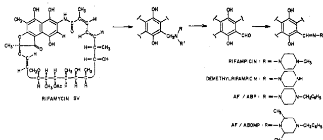
Figure 6. Biologically important compounds derived from rifamycin SV.
