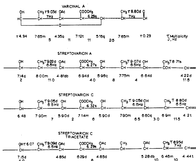
Figure 11. Chemical shifts and coupling of varicinal A protons and related protons in streptovaricins.
