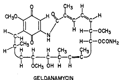
Figure 4. Structure assigned to geldanamycin.
